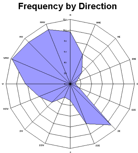
Figure 8. Wind rose displaying wind direction frequency.
