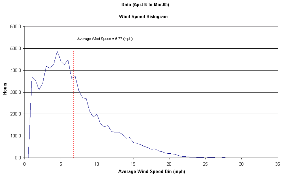
Figure E.6.4. Wind speed frequency over the year by # of hours.
