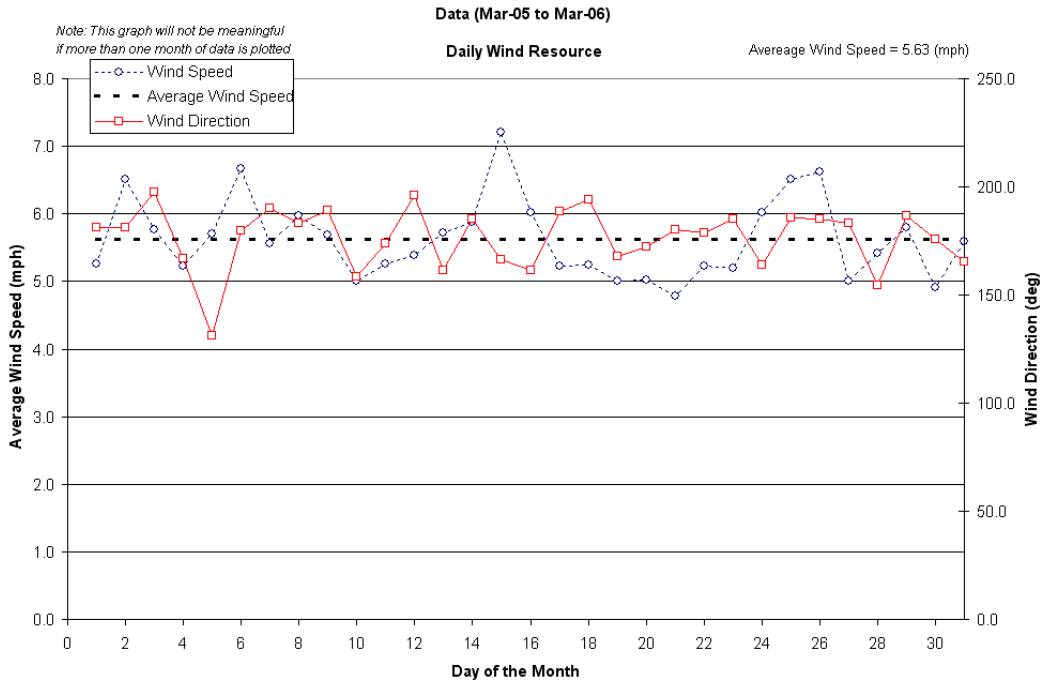
Figure E.2.6. Wind speed and direction averages by day of the month
