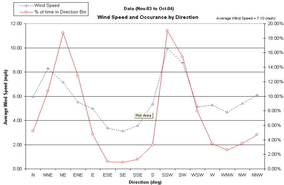
Figure 2. Average hourly wind speeds and directions throughout the year.
